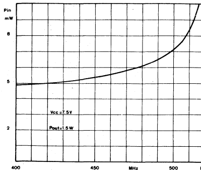
Figure 6. Input Power versus Frequency for 1.5 Watts Output
