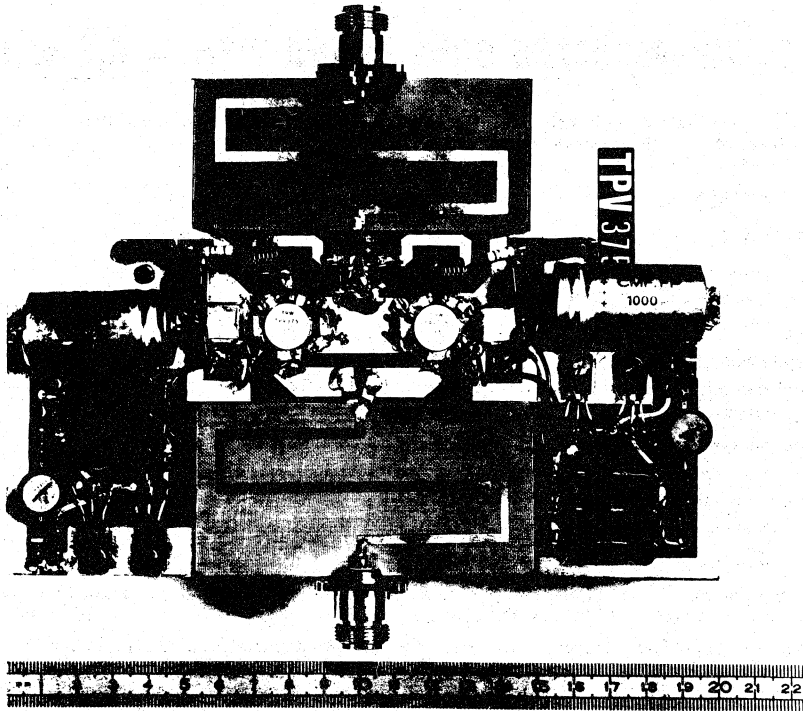
Figure 12. 160-240 MHz Amplifier
