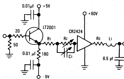
Figure 8. Experimental Circuit
