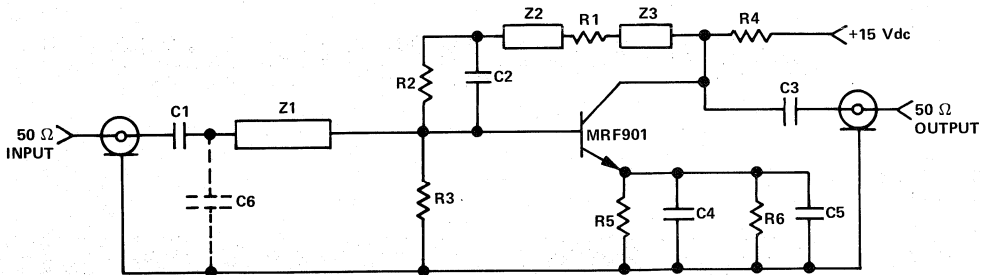
Figure 1. Schematic Diagram
