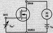
TEST CIRCUIT FOR I_{D(on)}
