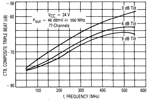
Figure 8. CTB versus Frequency/Tilt
