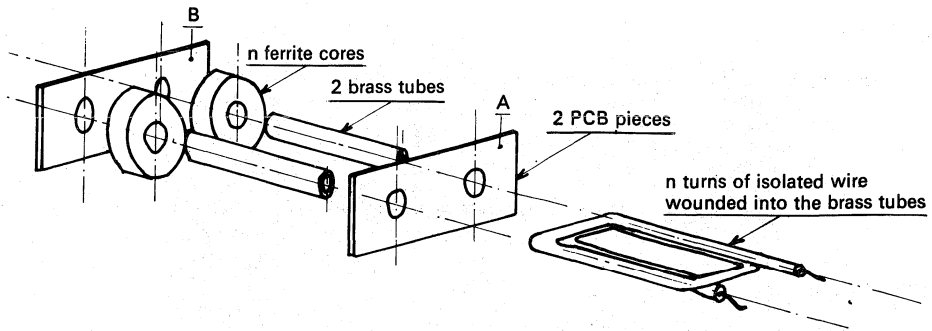
PARTS A AND B FOR T1 (INPUT)
