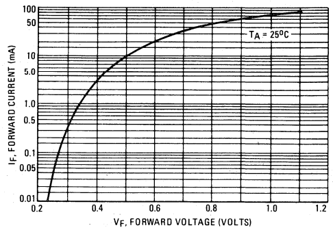
FIGURE 4 – FORWARD VOLTAGE
