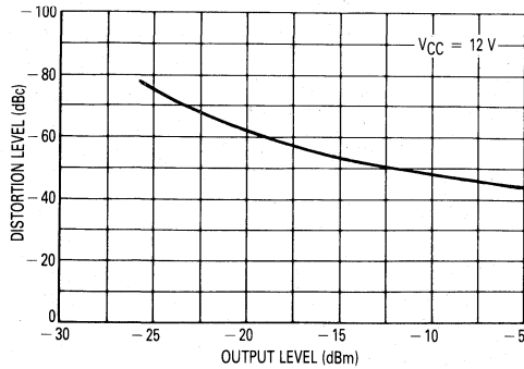
Figure 9. Second Order Intermodulation Distortion f_1 = 55.25 \text{ MHz (CH 2)} f_2 = 211.25 \text{ MHz (CH 13)} \text{Dist} = f_1 + f_2
