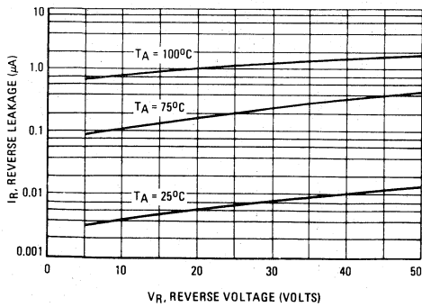
FIGURE 3 – REVERSE LEAKAGE
