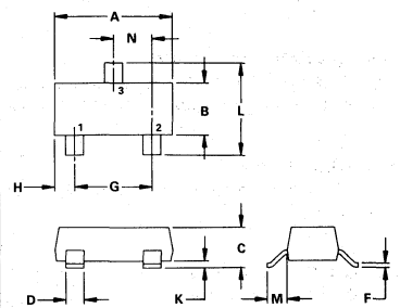
STYLE 8: PIN 1. ANODE 2. NO CONNECTION 3. CATHODE
