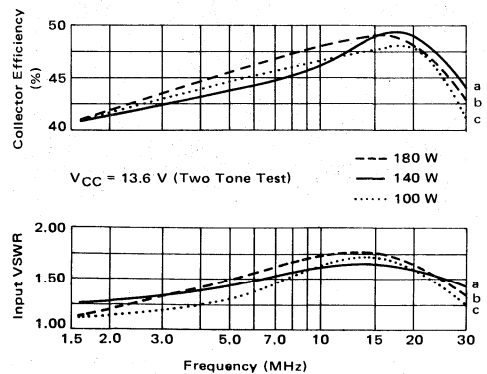
FIGURE 8 — Input VSWR and Collector Efficiency versus Frequency
