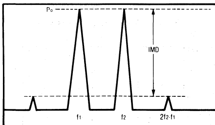
Figure 10. Intermodulation Test
