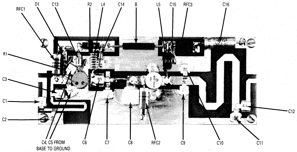
Figure 3. Parts Placement
