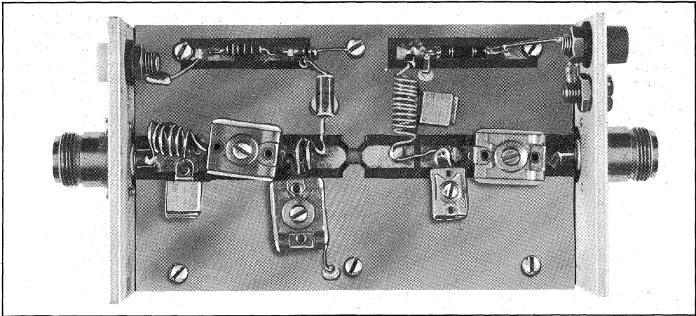
FIGURE A2 — Circuit Using Alumina/ Copper Socket
