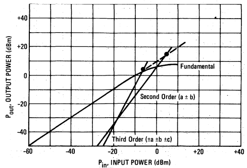
FIGURE 19 – SECOND AND THIRD ORDER INTERCEPT MWA210
