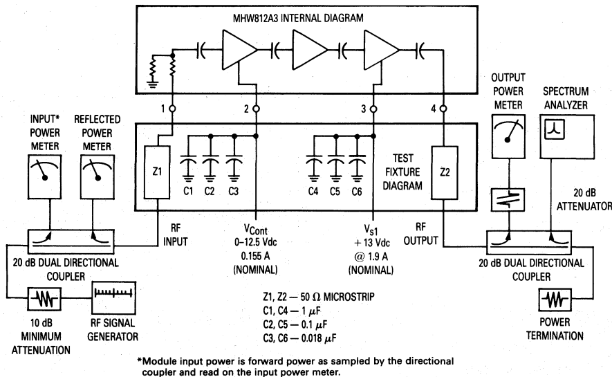
Figure 1. UHF Power Amplifier Test System Diagram
