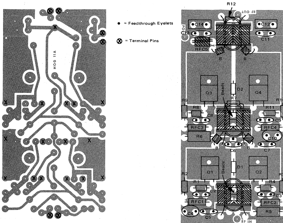
FIGURE 5 Component Layout Diagram of Low-Cost 20 W Amplifier
