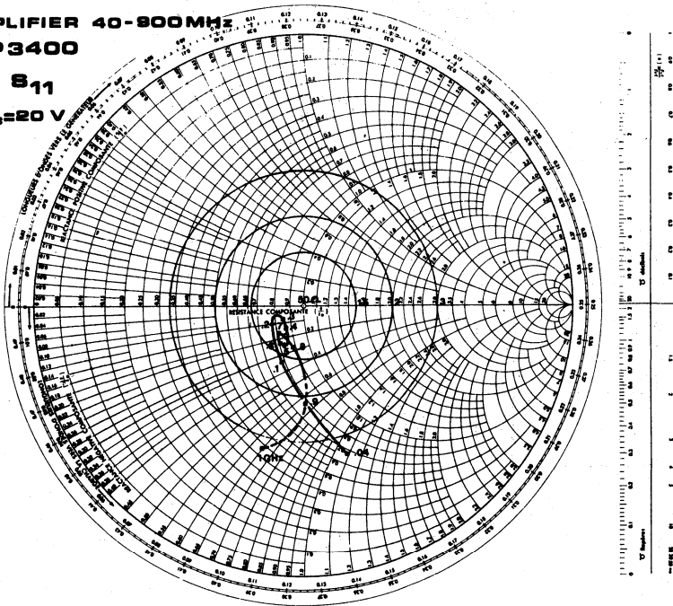
Figure 6. S 11 versus Frequency
