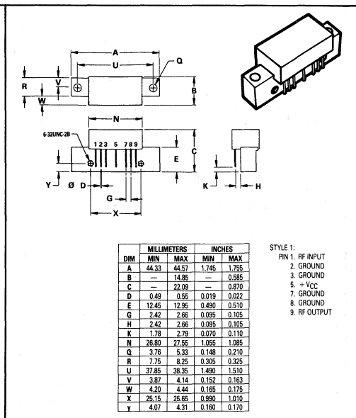
CASE 714F-01 (CA, POS. SUPPLY)
