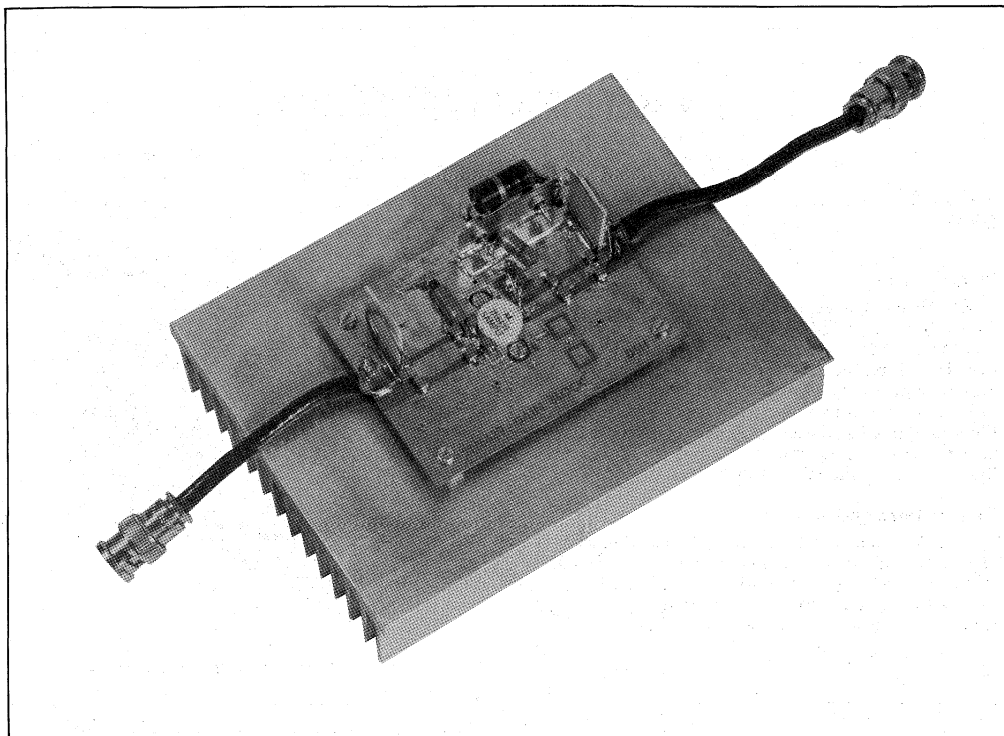
FIGURE 8 — Amplifier Assembly
