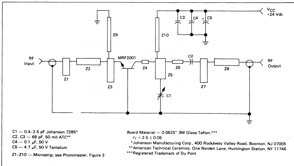
FIGURE 2 — Schematic Diagram
