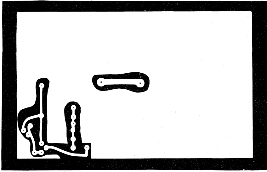
FIGURE 10—Photomaster (Positive)
