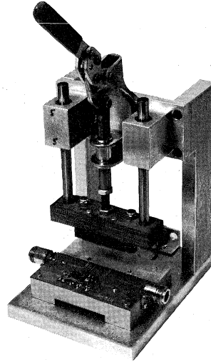
Figure 14. Test Fixture Assembly
