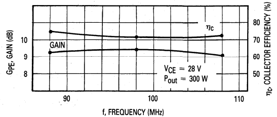
Figure 4. Gain and Efficiency versus Frequency
