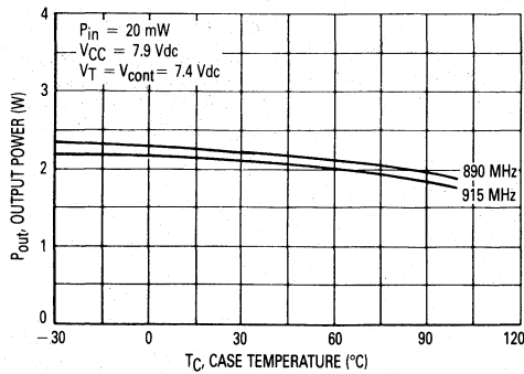
Figure 11. Output Power versus Case Temperature
