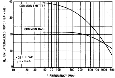
FIGURE 8 – UNILATERIALIZED POWER GAIN versus FREQUENCY
