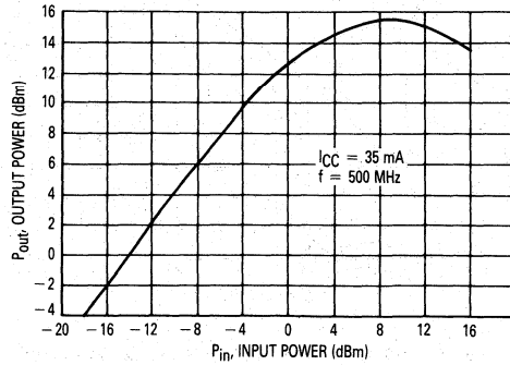
Figure 6. Output Power versus Input Power
