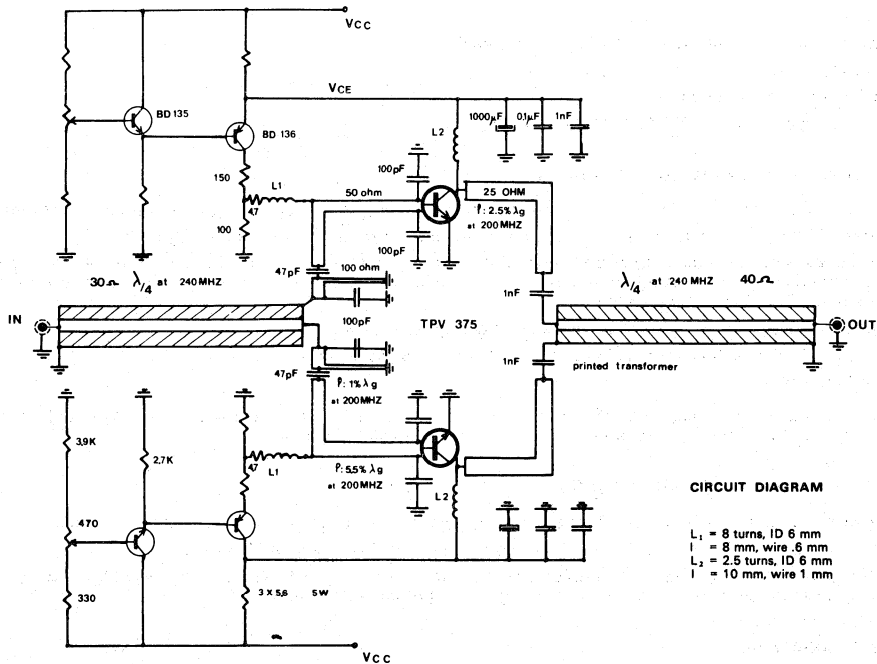
Figure 2. Circuit Diagram
