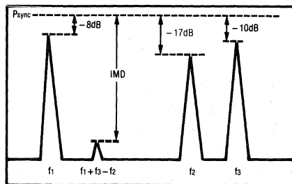
Figure 12. 3-Tone TV Intermodulation Test
