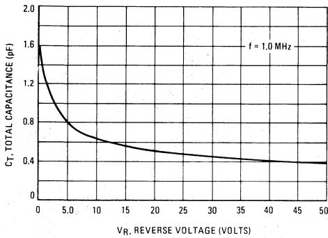
FIGURE 1 – TOTAL CAPACITANCE
