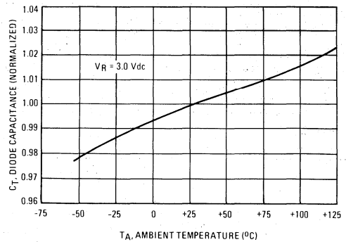
FIGURE 3 – DIODE CAPACITANCE
