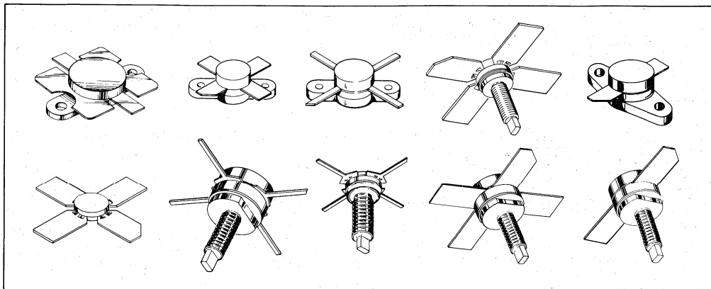
FIGURE 1 — SOE Packages
