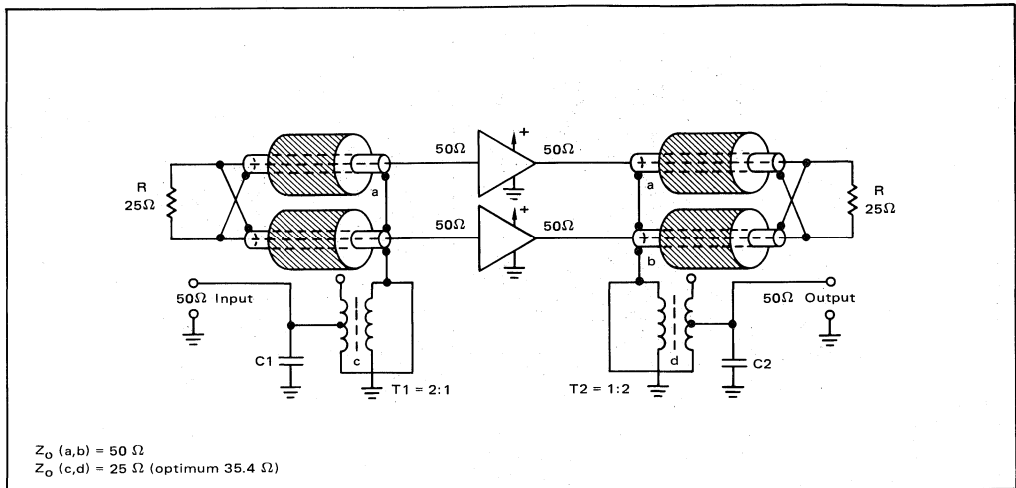
FIGURE 10 — Two-Port Hybrid System
