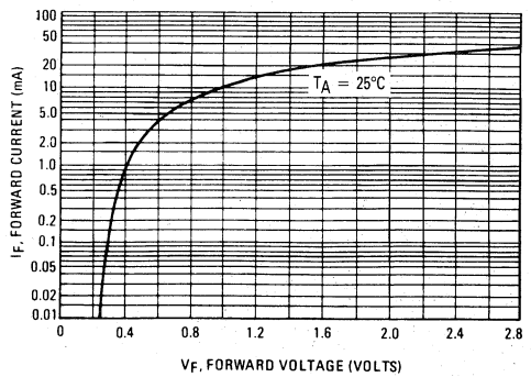
FIGURE 4 – FORWARD VOLTAGE
