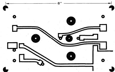
FIGURE 25 - Bottom PC Board Pattern
