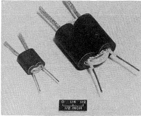
Transformer Construction
