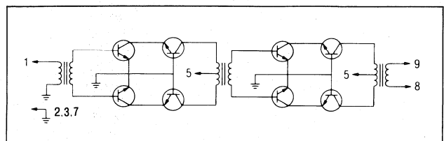
Figure 2. Double Parallel/Cascade Circuit
