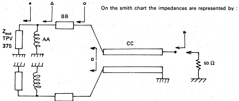
Figure 12. 160-240 MHz Amplifier
