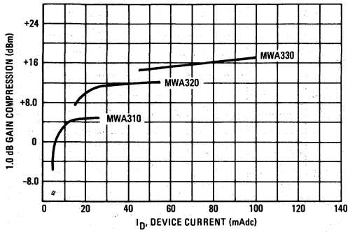
FIGURE 17 – 1.0 dB GAIN COMPRESSION versus DEVICE CURRENT versus DEVICE CURRENT f = 1000 \text{ MHz}
