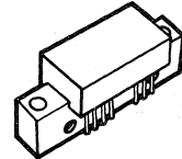
CA (NEG. SUPPLY) CASE 714H-01, STYLE 1 CA5501R
