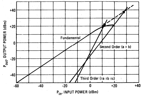
FIGURE 23 – INTERMODULATION DISTORTION versus POWER OUTPUT MWA220
