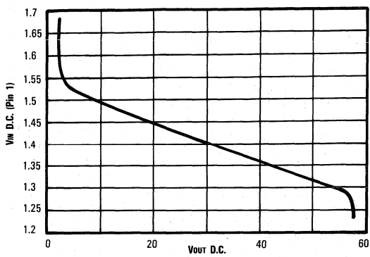
Figure 5. Voltage Ratio at Port 1
