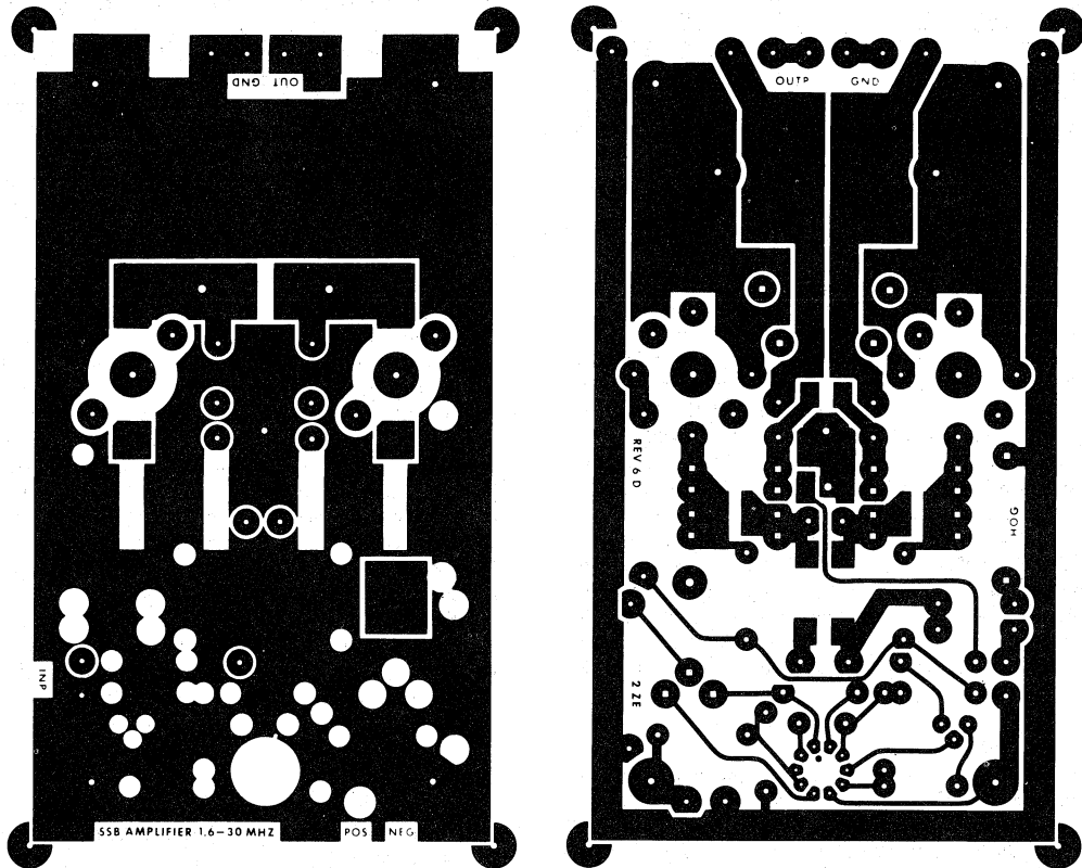
FIGURE 11 — Printed Circuit Board Layout
