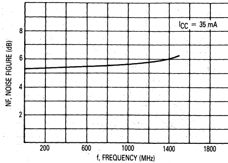
Figure 2. Noise Figure versus Frequency
