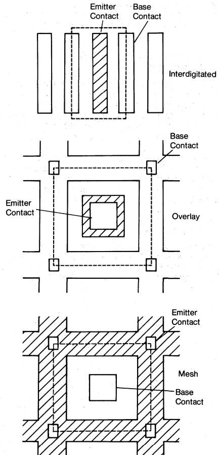
Figure 5. Typical Transistor Configurations
