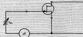
FIGURE 12a — V_{(BR)GSS} Test Circuit
