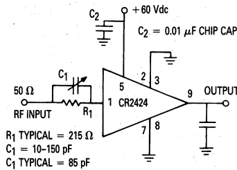
Figure 5. CRT Amplifier Test Circuit
