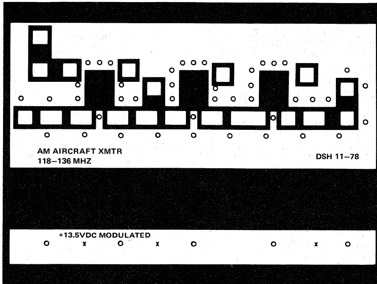
FIGURE 6 – Photomaster
