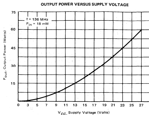
P_{out} is initially set at the carrier power of 15 watts at 13.5 Vdc, then the supply voltage is varied from 0 to 27 Vdc keeping P_{in} constant. This demonstrates the peak power output capability of the transmitter P.A.
