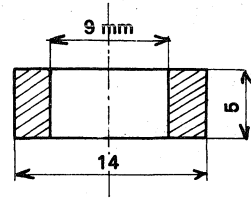
Figure 6. Output Ferrite Toroid
