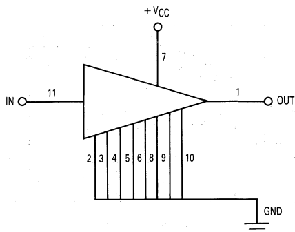
Figure 11. Amplifier Configuration
