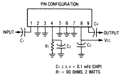
Figure 13. External Connections
