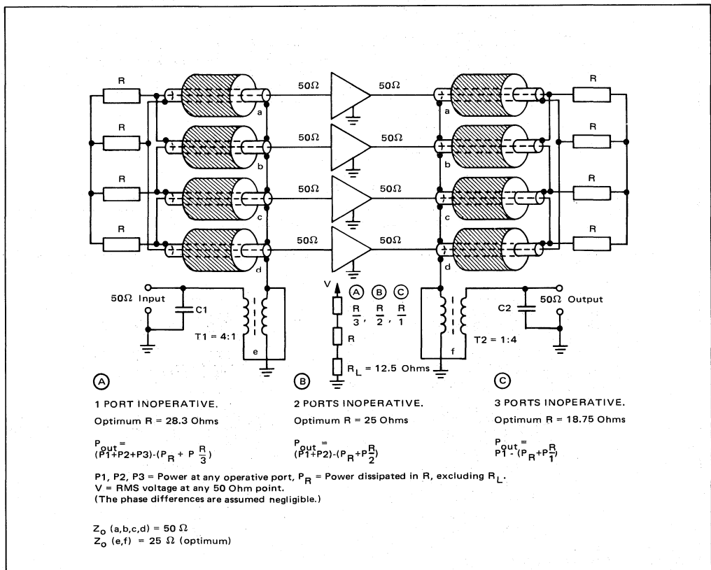
FIGURE 11 — Four-Port Hybrid System
