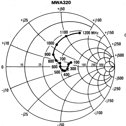
FIGURE 15 – OUTPUT IMPEDANCE versus FREQUENCY
