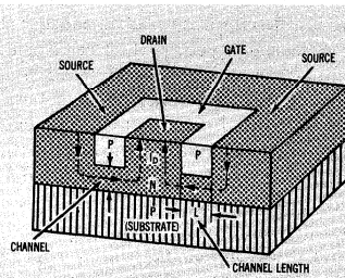
FIGURE 3 - Junction FET with Single-Ended Geometry
