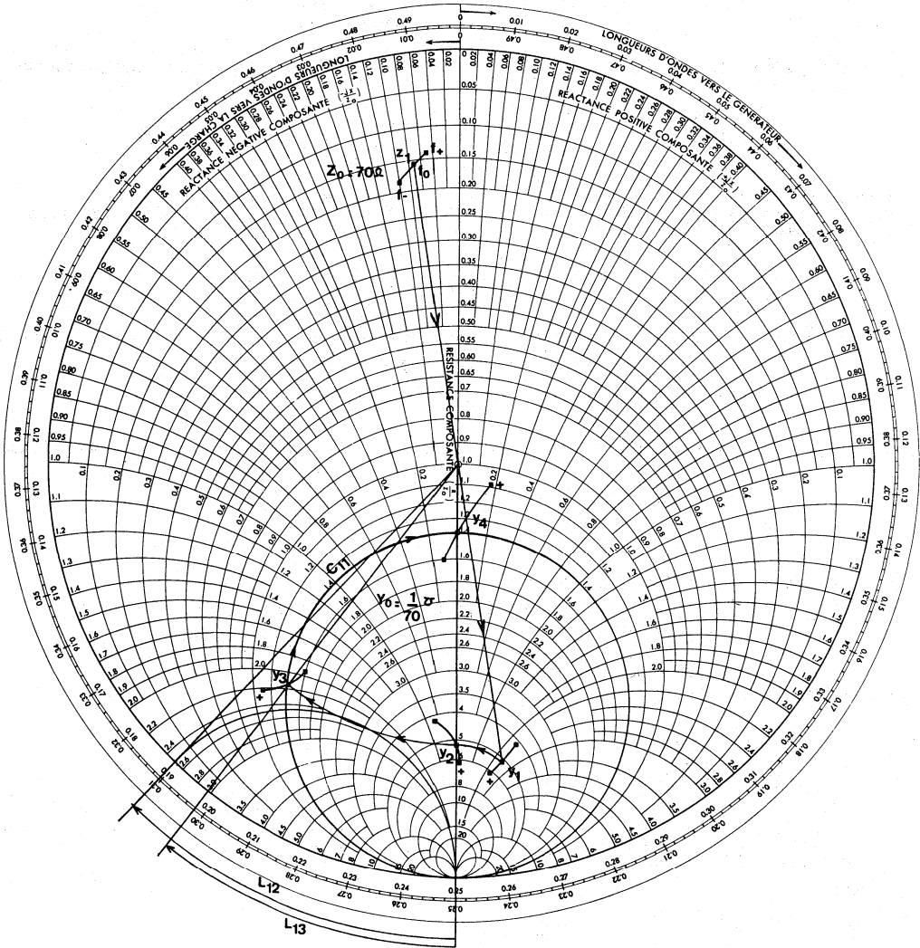
Figure 3. Smith Chart Calculations for Output Matching Network
