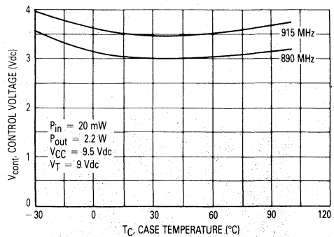
Figure 10. Control Voltage versus Case Temperature
