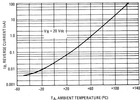
FIGURE 3 — LEAKAGE CURRENT
