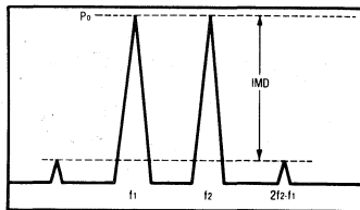
Figure 1. Intermodulation Test
