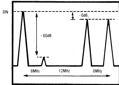
Figure 2. DIN45004B Test
