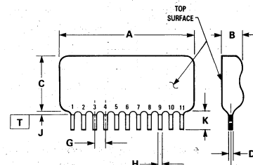
STYLE 1: PIN 1 — OUTPUT 7 — V CC 11 — INPUT 2,3,4,5,6 8,9,10 — GROUND
