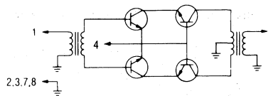
Figure 11. Functional Schematic
