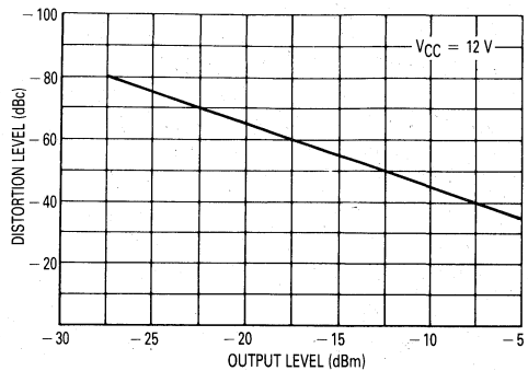
Figure 10. Third Order Intermodulation Distortion f_1 = 199.25 \text{ MHz (CH 11)} f_2 = 211.25 \text{ MHz (CH 13)} \text{Dist} = 2f_2 - f_1
