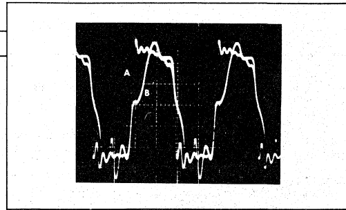
FIGURE 6. Driver output waveform at 25 MHz. A without a load. B loaded by the P.A. FET gate. Results of the uneven gate capacitance distribution versus gate and drain voltage can be noticed in B. 10 nS and 2v/div.
