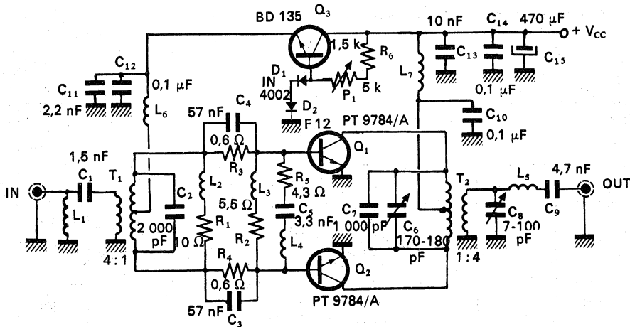
Figure 1. Broadband Push-Pull Amplifier
