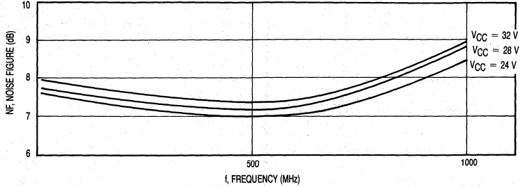
Figure 9. Noise Figure versus Frequency
