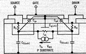
FIGURE 6 — Equivalent Circuit of Enhancement-Mode MOSFET
