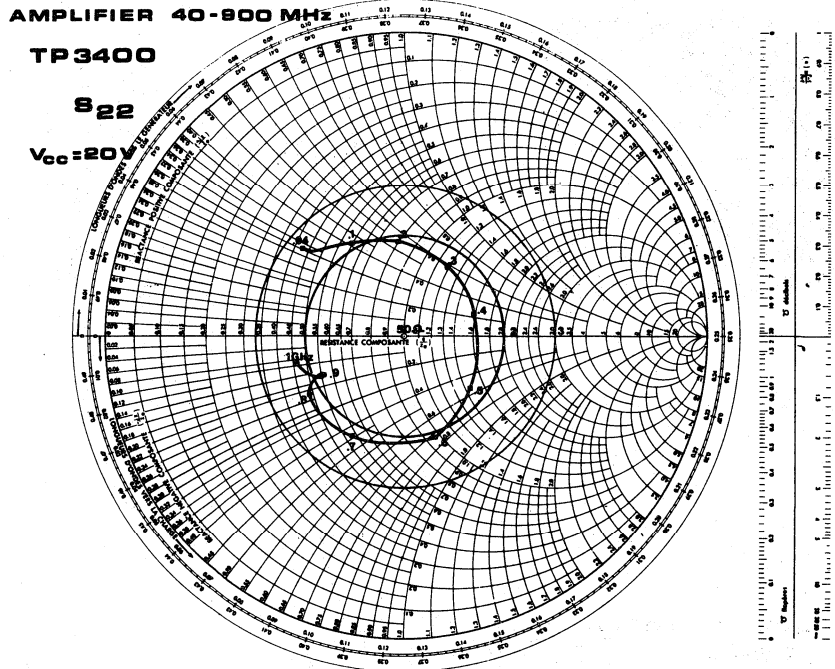
Figure 7. S_{22} versus Frequency
