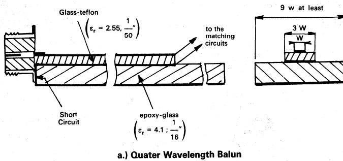
a.) Quater Wavelength Balun
