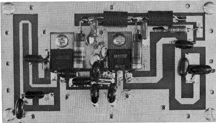
FIGURE 2 — 136-160 MHz Amplifier
