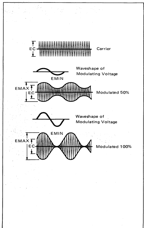
FIGURE 10 — Amplitude Modulation Waveforms
