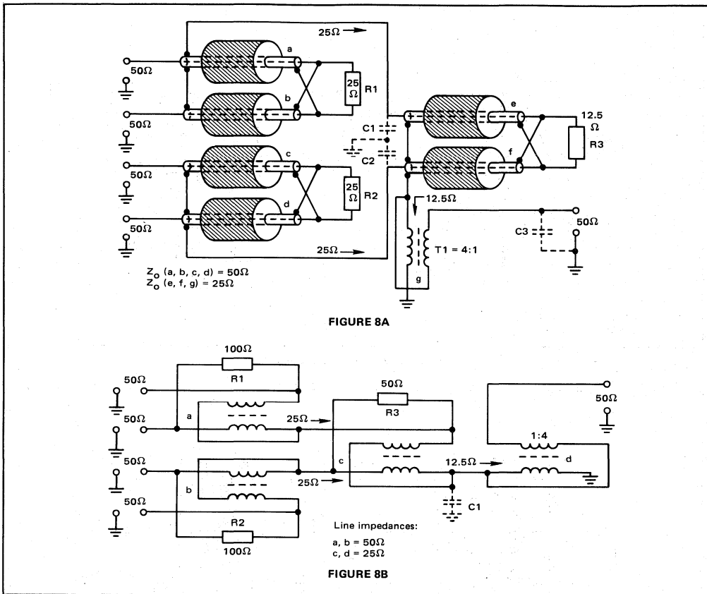
FIGURE 8 – Four Port "Totem Pole" Structure
