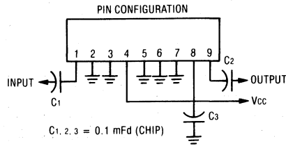
Figure 3. External Connections
