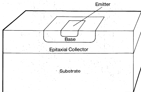
Figure 3. Planar-Epitaxial Technology
