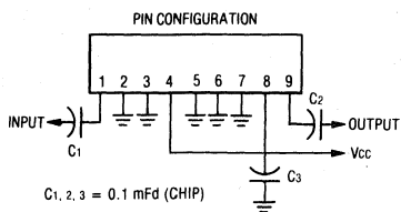
Figure 13. External Connections
