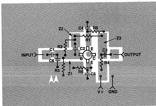
Figure 5. Parts Layout
