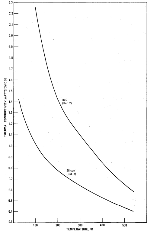
FIGURE 3 – Thermal Conductivity
