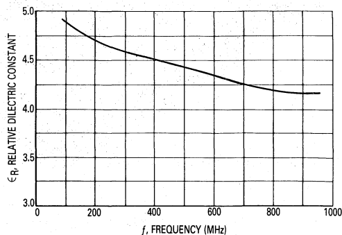
Figure 3 — Relative Dielectric Constant (G-10) versus Frequency
