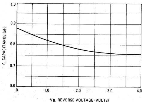
FIGURE 3 – CAPACITANCE
