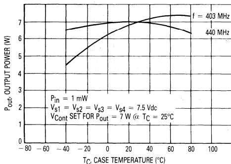
Figure 6. Output Power versus Case Temperature
