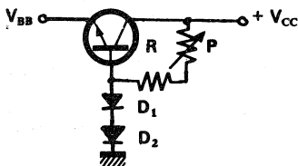
Figure 14. Bias Circuit
