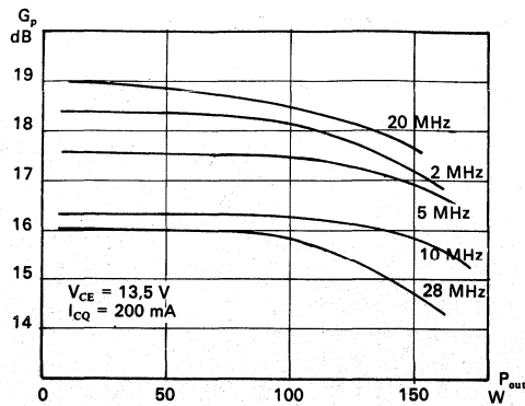
Figure 19. Gain versus Input Power
