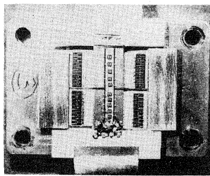
Fig. 4. In this experimental RF MOSFET four die are connected in parallel. Chip-type silicon gate resistors are located at the center.
