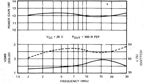
Figure 1 — Collector Efficiency, Power Gain and VSWR vs Frequency
