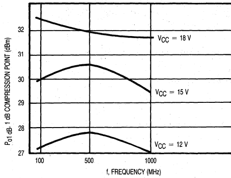
Figure 3. 1 dB Compression versus Frequency
