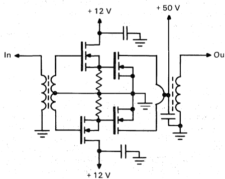
FIGURE 7 — A Typical Power MOSFET Class D RF Amplifier, Arranged in Push-Pull Configuration
