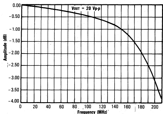
Figure 6. Frequency Response of CR2424
