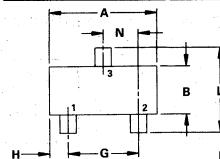
CASE 182-02 TO-226AC MBD101
