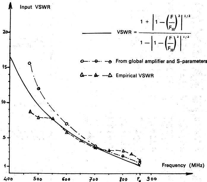
Figure 1. Input VSWR
