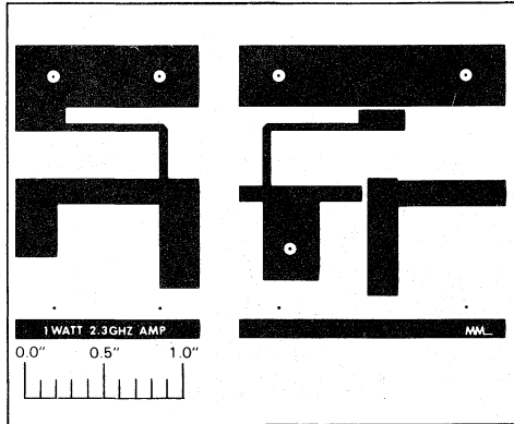
NOTE: The Printed Circuit Board shown is 75% of the original.
