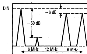
Figure 2. DIN45004B Test
