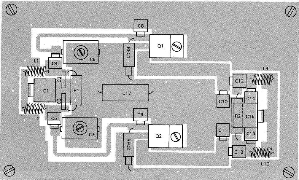
FIGURE 3 — Component Placement
