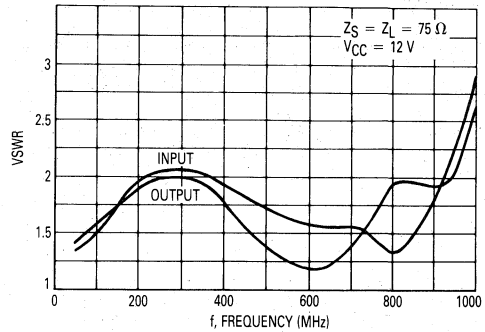
Figure 8. Input and Output VSWR versus Frequency
