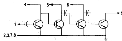
Figure 11. External Connections
