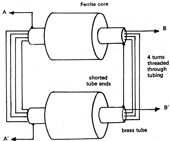
Figure 5. Transformer Construction
