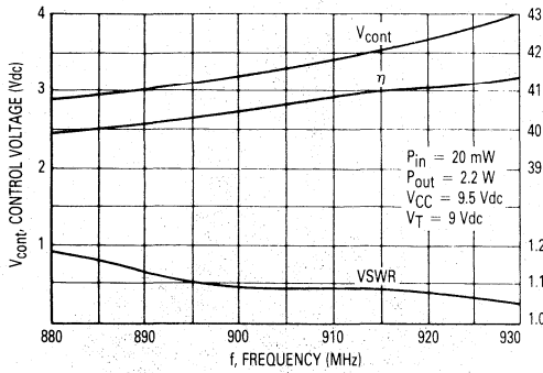
Figure 7. Control Voltage, Efficiency, and VSWR versus Frequency
