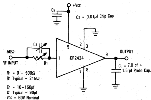
Figure 7. Test Circuit
