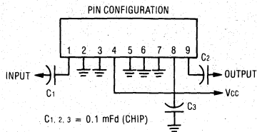
Figure 13. External Connections
