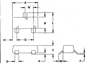
CASE 182-02 TO-226AC MV209
