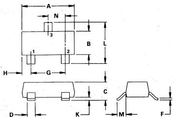
STYLE 8: PIN 1. ANODE 2. NO CONNECTION 3. CATHODE
