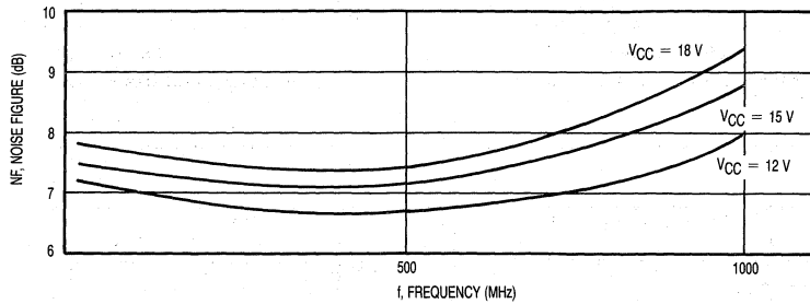
Figure 9. Noise Figure versus Frequency
