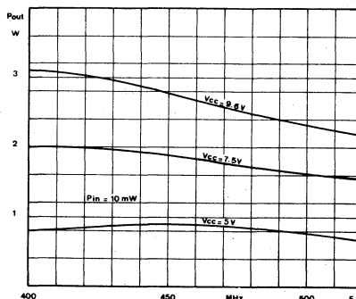
Figure 8. Output Power versus Frequency and Voltage Supply
