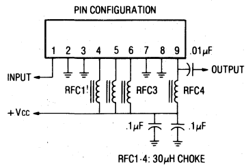
Figure 12. External Connections
