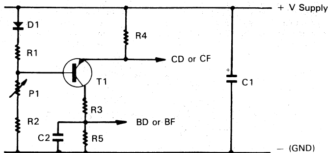
Figure 3. Electrical Circuit
