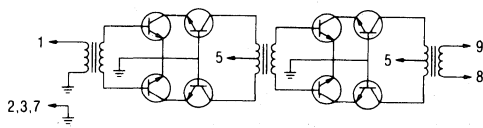
Figure 10. Functional Schematic
