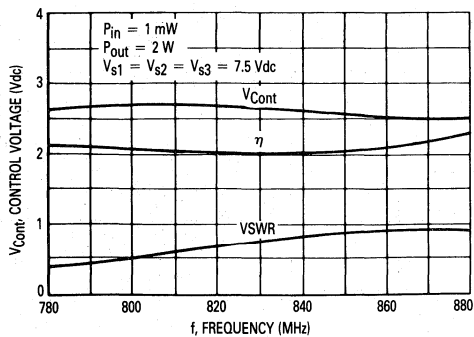
Figure 2. Control Voltage, Efficiency and VSWR versus Frequency
