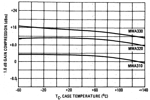
FIGURE 18 – 1.0 dB GAIN COMPRESSION versus CASE TEMPERATURE versus CASE TEMPERATURE f = 1000 \text{ MHz}
