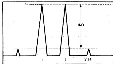
Figure 11. Intermodulation Test
