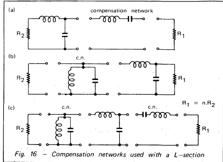
Fig. 16 - Compensation networks used with a L-section
