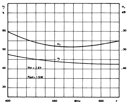
Figure 7. Efficiency and Harmonic Rejection versus Frequency
