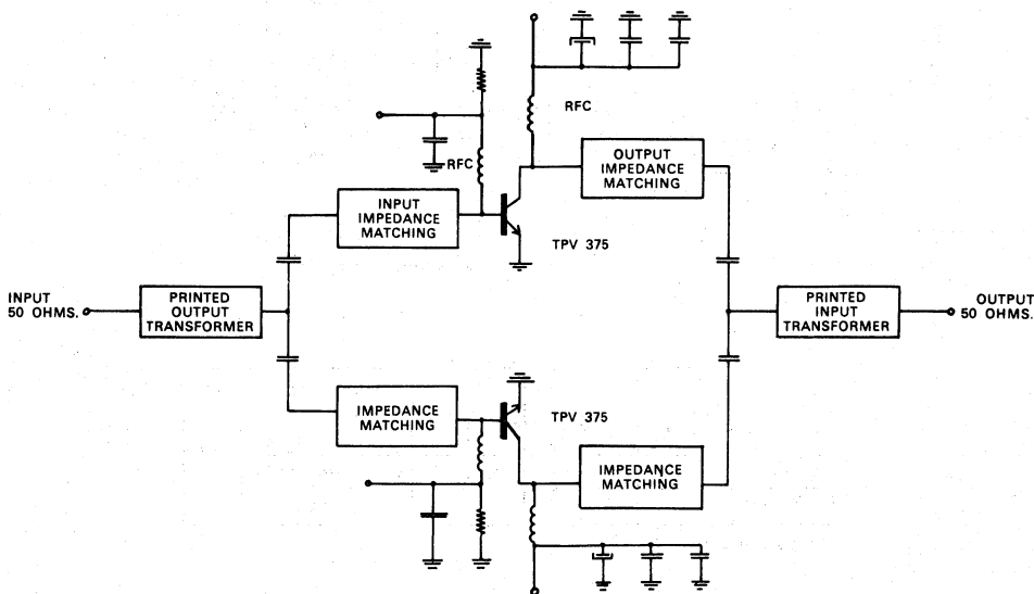
Figure 1. Push-Pull Circuit
