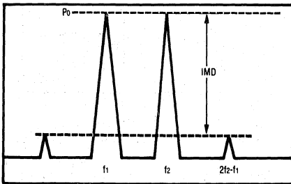
Figure 11. 2-Tone Intermodulation Test
