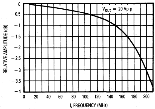
Figure 4. Frequency Response
