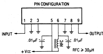
Figure 12. External Connections
