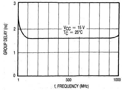
Figure 8. Group Delay versus Frequency
