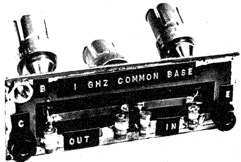
FIGURE 9 – 1 GHz AMPLIFIER
