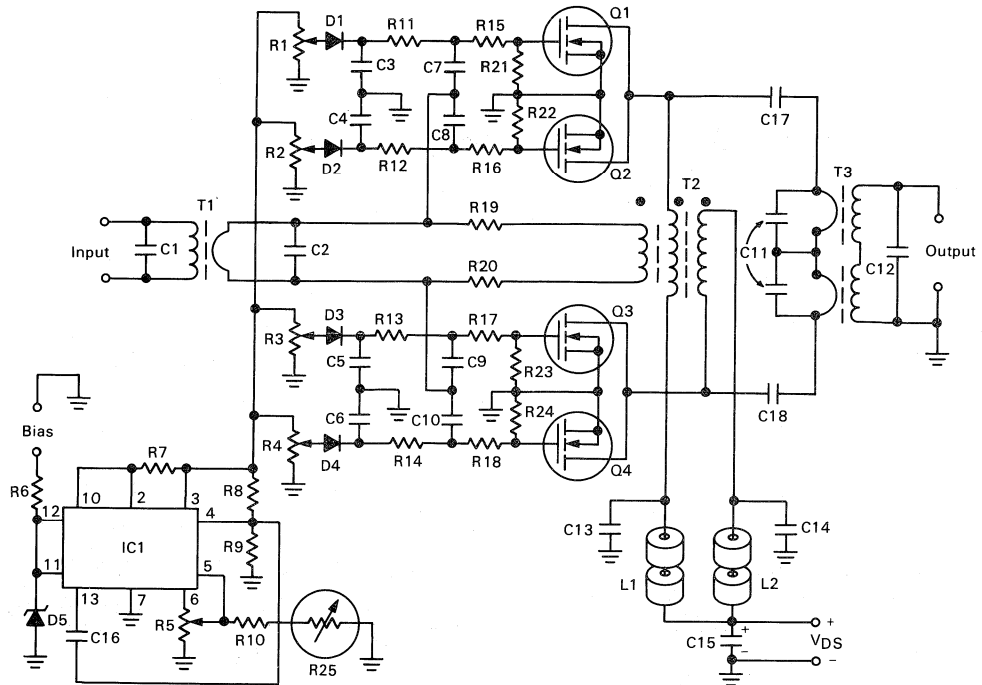
FIGURE 2 — Detailed Schematic
