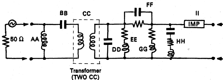
Figure 12. RF Equivalent Input Circuit
