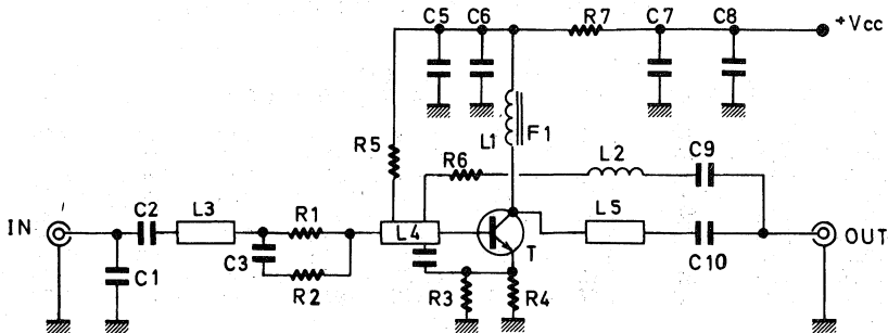
Figure 3. Circuit Schematic
