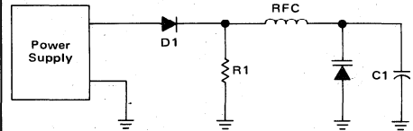
METHOD TWO — Schematic Diagram
